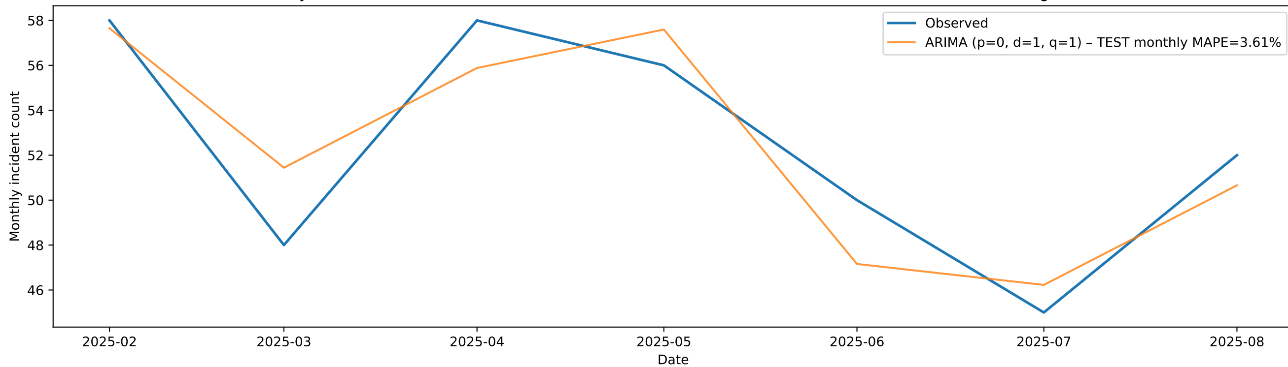
Monthly Traffic Incidents in Anadolu Street: Best Time-series Model vs Observed (TEST, Feb 2025-Aug 2025)
