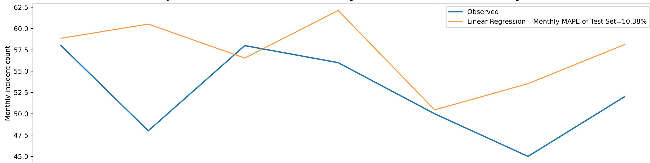
Monthly Traffic Incidents in Anadolu Street: Best Time-series Model vs Observed (TEST, Feb 2025-Aug 2025)
